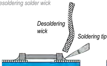
Solder melting and removal with a desoldering solder wick
